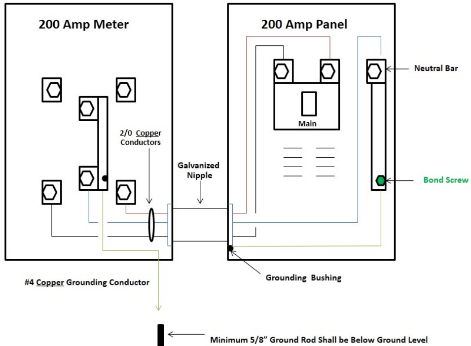
200 Amp UnderGround Meter Loop with Galvanized Nipple
